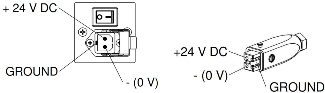
Figure 5, 24 V-input Manager IQ Easy
