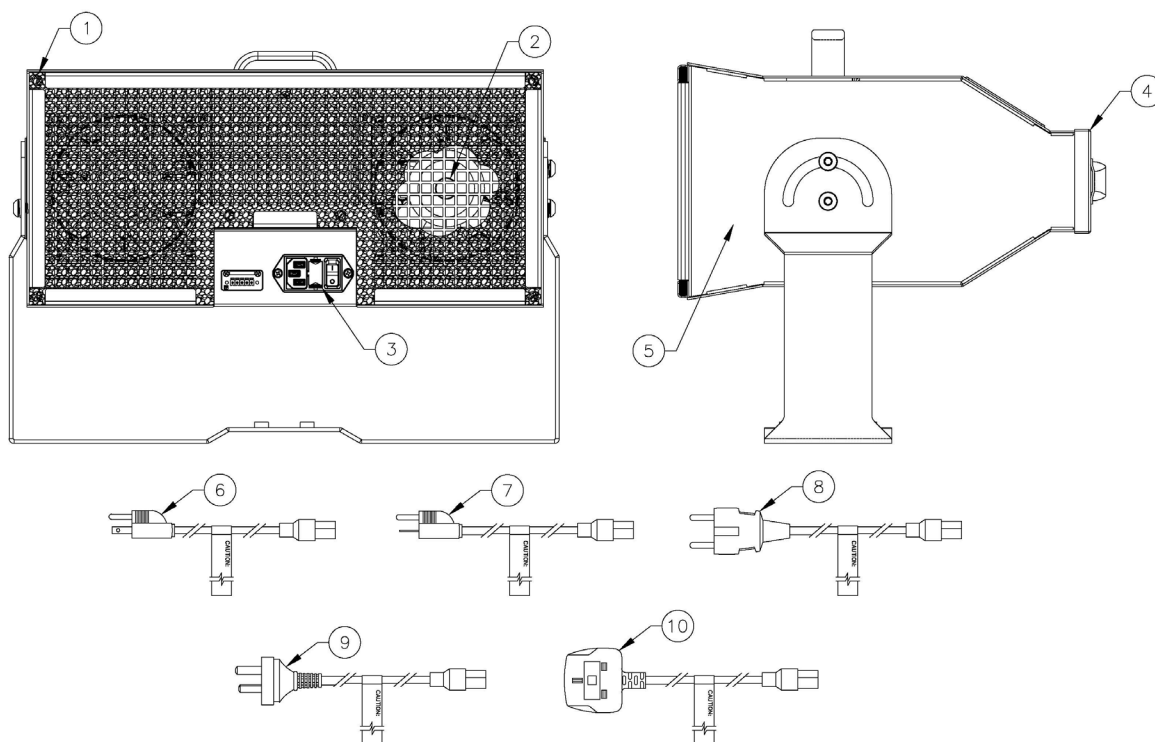
Figure 11. Replacement Parts
