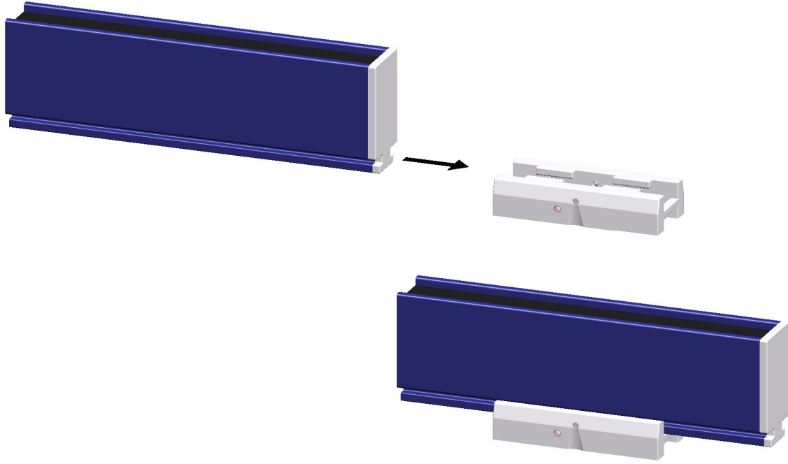
Example: total Anti Static Bar to be slid on fixed bracket
